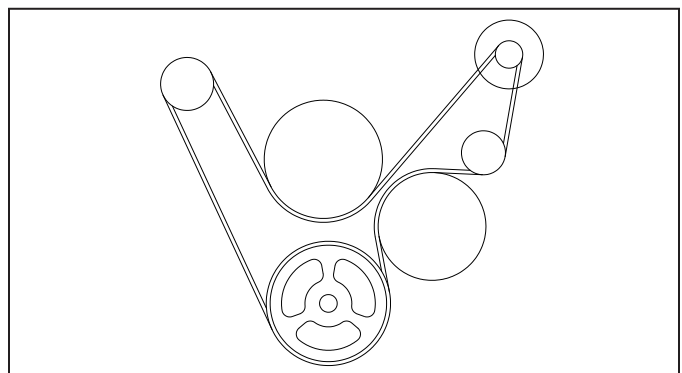
6.2L SC Accessory Drive Belt Configuration
