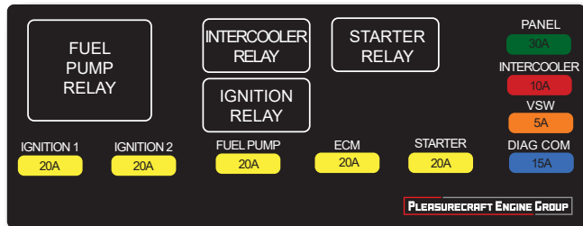
Typical Fuse Block Layout
